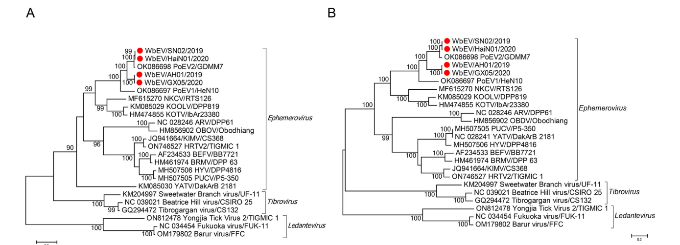
Fig. 3. Phylogenetic trees based on full length of N (A) and L (B) protein sequences of representative species of 3 genera within the Rhabdoviridae family. Four WbEV strains are marked with red dots. The phylogenetic tree was constructed by MEGA v7.0 using the maximum likelihood method with 1000 bootstrap replicates, and the best fitting substitution models was LG + G + I and LG + G + I + F, respectively. The bootstrap support values greater than 70% are shown at relevant nodes.
